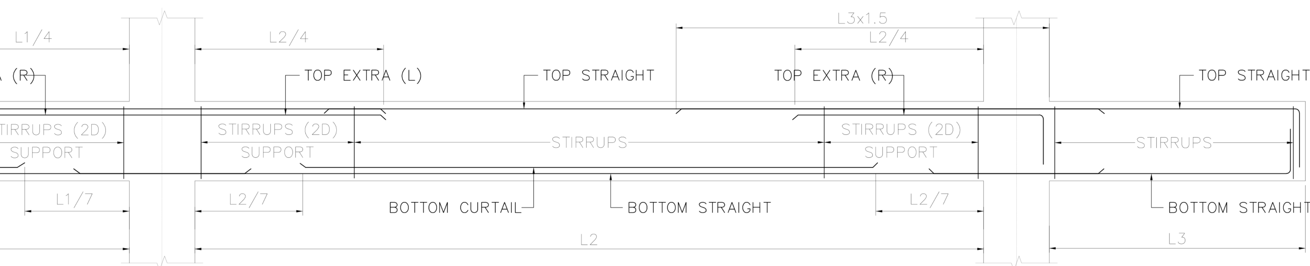
OF SPECIAL CONFINING REINFORCEMENT REQUIREMENT FOR BEAM REINFORCEMENT
