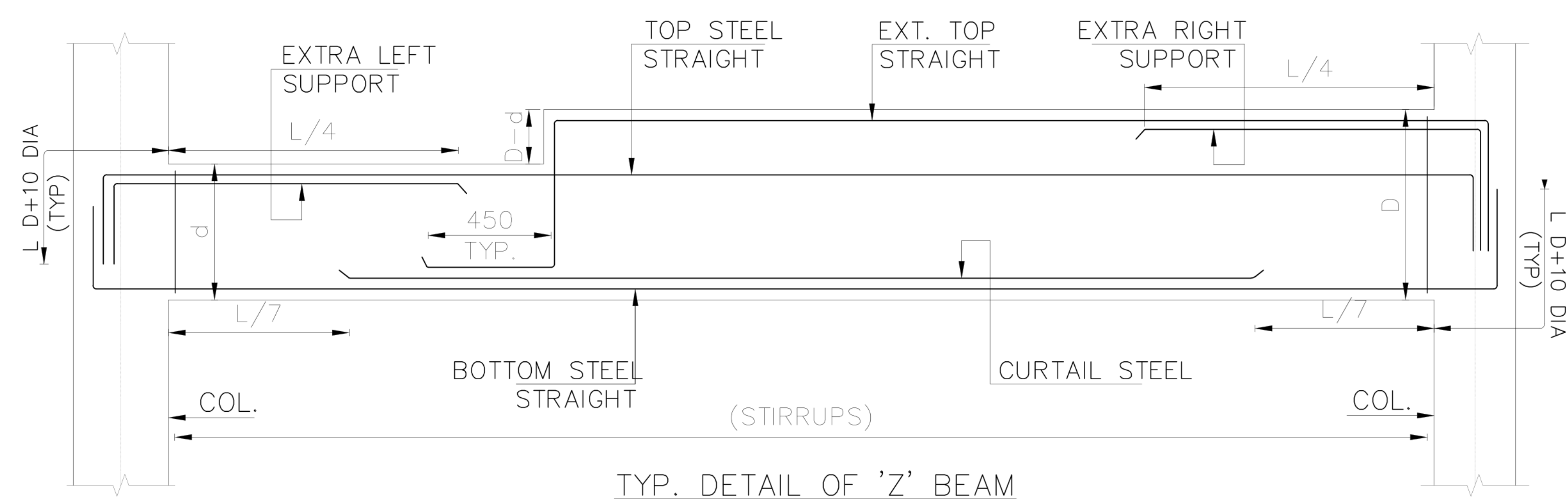
TYP. DETAIL OF 'Z' BEAM
